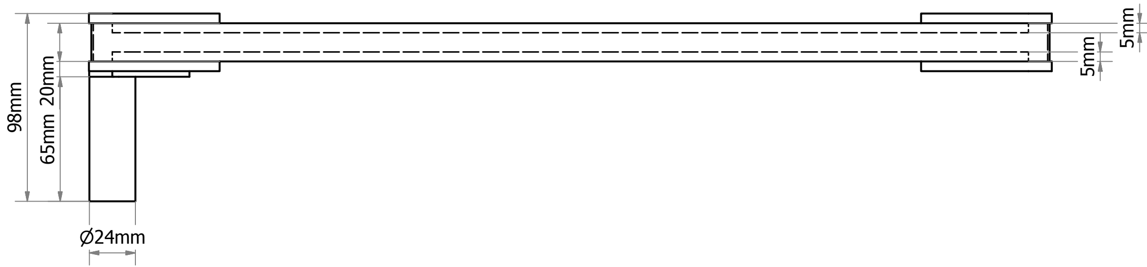
FRONT VIEW
